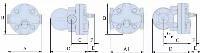
FTC32 DN15-20
