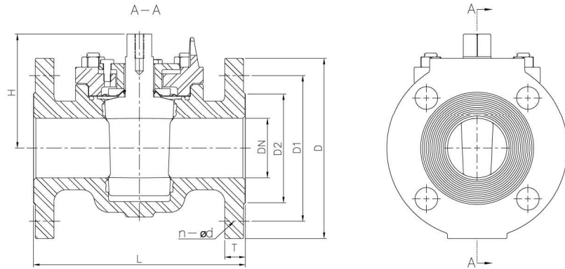
Flanged End / Class 150 / 2 way - Fig. P11F1 Sleeved Plug Valve
