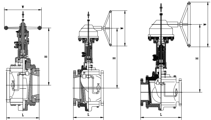
DBB式旋塞阀 DBB plug valve
