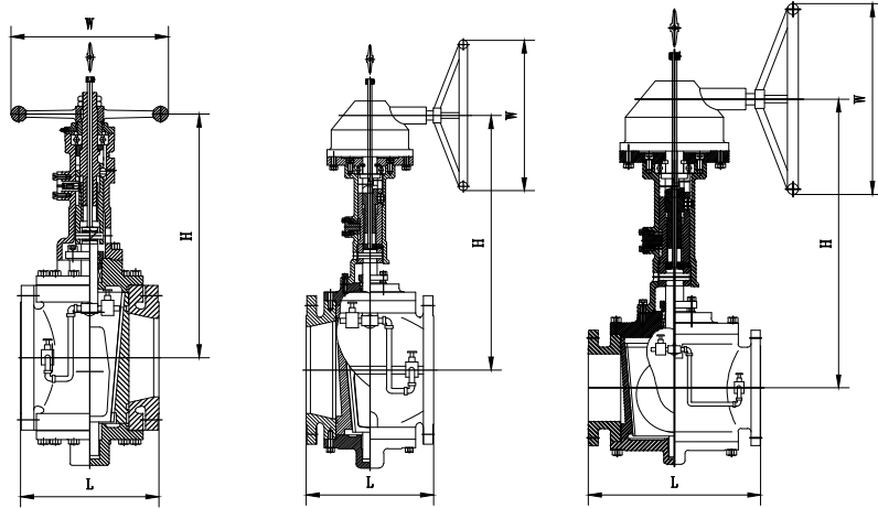
DBB式旋塞阀 DBB plug valve
