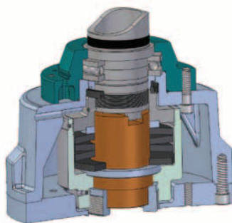
Rotork thrust compensator.
